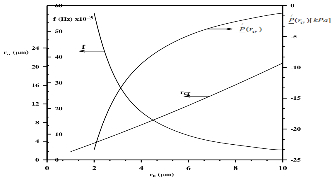
Fig.1 Variation of critical cavitation nuclei radius ( r_{cr} ), critical pressure at the nuclei surface ( \underline{p}(r_{cr}) ), and the frequency (f) of the liquid contains gas nuclei with various initial nuclei radii ( r_0 ).
