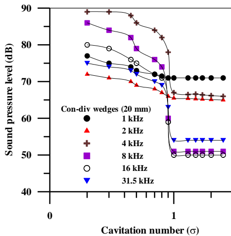
Fig. 5 Variation of sound pressure level with cavitation number at various frequencies for 20 mm con-div wedges.
