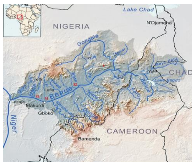
Figure 1. Benue River Basin showing sampling sites along the Benue River basin. Sampling site 1 (S1) ( 7^{\circ}44'N , 8^{\circ}32'E ) Benue River. Sampling site 2 (S2) ( 8^{\circ}26'N , 10^{\circ}05'E ) Discharge of Wase river into the Benue River and Sampling site 3 (S3) ( 7^{\circ}59'N , 7^{\circ}55'E ) Discharge of the Mada river into Benue River. Source google maps 2019.
