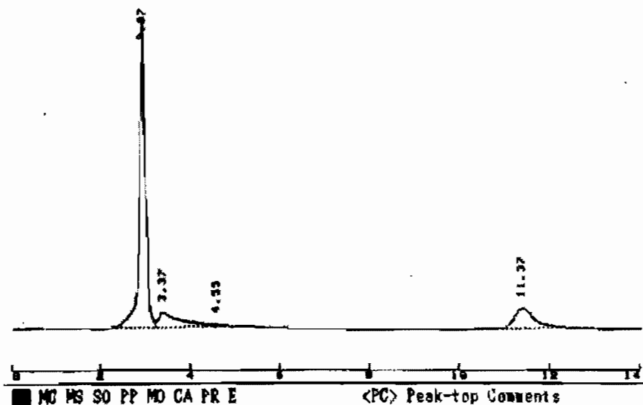
Figure (3): Chromatograph of oxytetracycline concentration mg/ml of milk after 24 hr from first day of drug administration
