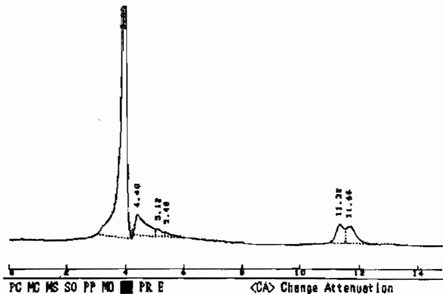
Figure (4): Chromatograph of oxytetracycline concentration after boiling of milk at 24 hr from drug administration.
