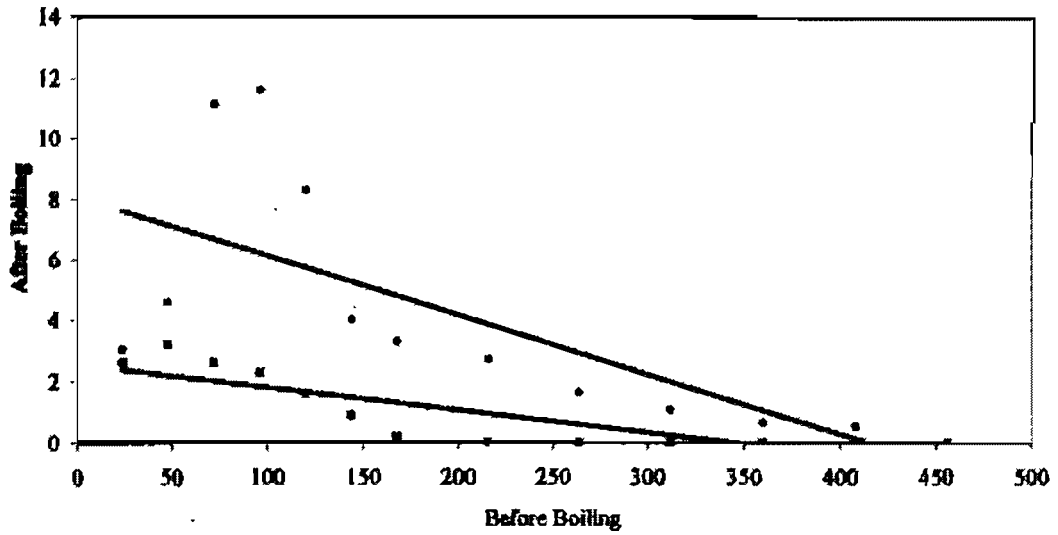
Figure (1): Oxytetracycline residues and the effect of boiling in cow's milk after intramuscular administration at a dose of (20 mg/Kg B.W.) for three successive days
