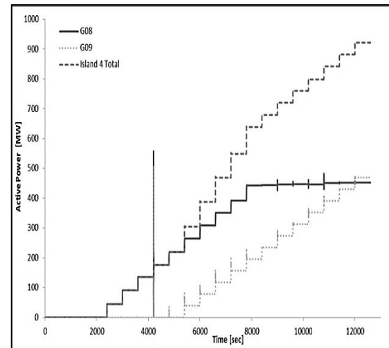
Fig.2: Power generation at island 4
