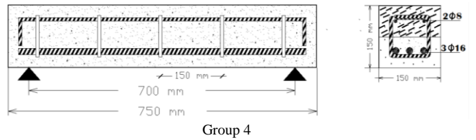
Figure (1): from group 1 to 4: Geometrical and reinforcement details of the tested beams.
