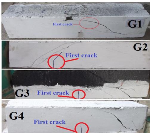
Figure (4) the mode of failure for all tested specimens.
