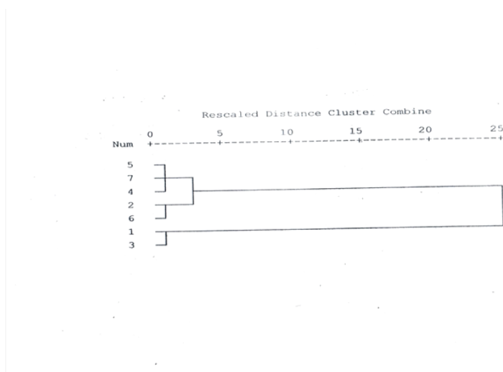
Fig1. Phenogram based on average linkage cluster analysis of reaction classes profiles of seven commercial cotton cultivars when they were inoculated with isolates of FOV races 3. The tested cultivars were Giza90(1), Giza80(2), Giza87(3), Giza92(4), Giza86(5), Giza45(6) and Giza86(7)
