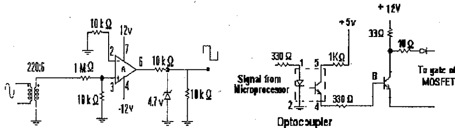
Fig.8b Synchronization circuit Fig. 8c MOSFET driver circuit
