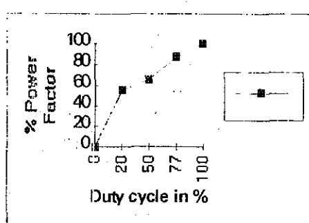
Fig.17 Power factor variation against duty cycle
