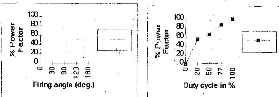
Fig. 15 Power factor against firing angle
