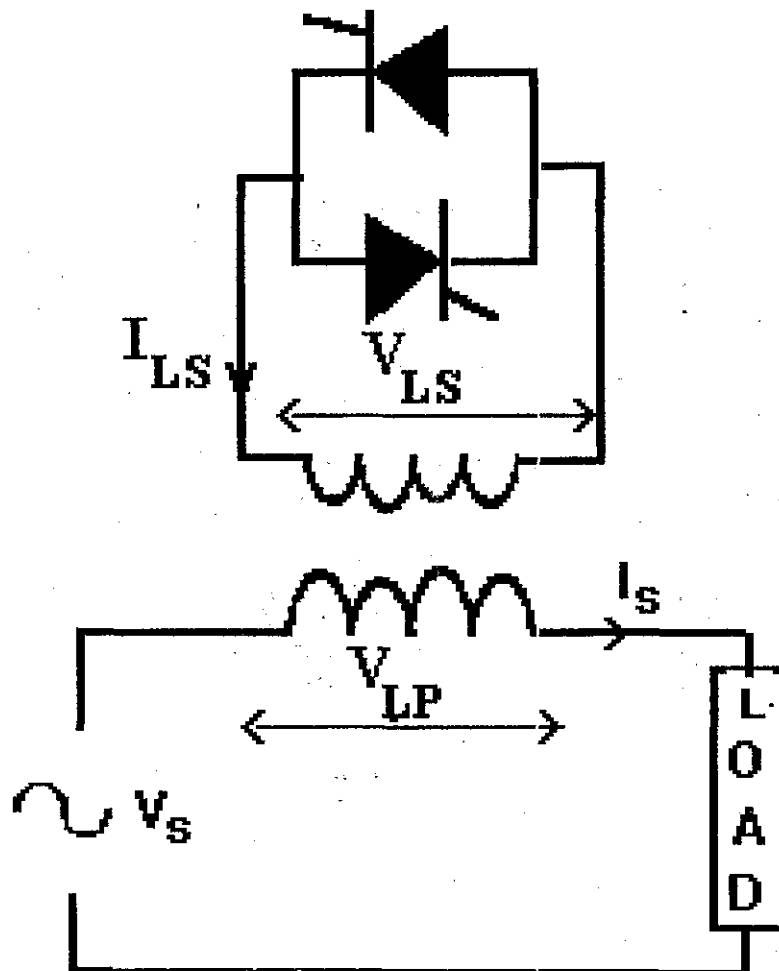
Fig. 1 Schematic diagram of first proposed system
