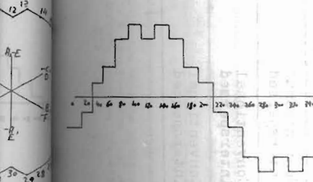
Fig. (3) Derivation of space MMF for, a six-phase winding with \delta = 60^\circ , unity-pitch, S = 18 , Q = 3 slots for two cases I, and II. (a) Stator-coil currents for double pole pitch. (b) Goerge's vector diagram. (c) The space MMF waveform.
