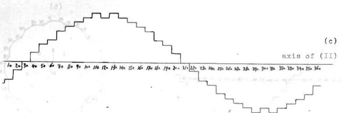
Fig. (2) Derivation of space MMF for, a six-phase winding with \delta = 60^\circ , unity-pitch, S = 36 , \alpha = 6 slots for two cases I, and II. (a) Stator-coil currents for double pole pitch. (b) George's vector diagram. (c) The space MMF waveform.
