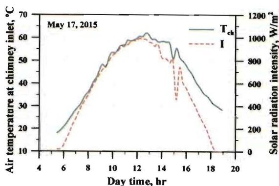
Figure 4, Air temperature at chimney inlet and solar radiation during May 17, 2015
