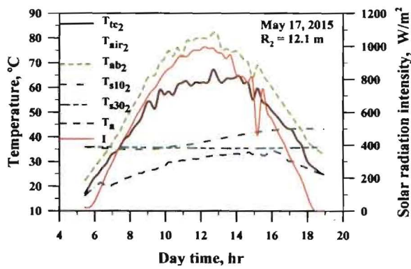
Figure 6 Temperature sensors records at R_2=12.1 m on May 17, 2015
