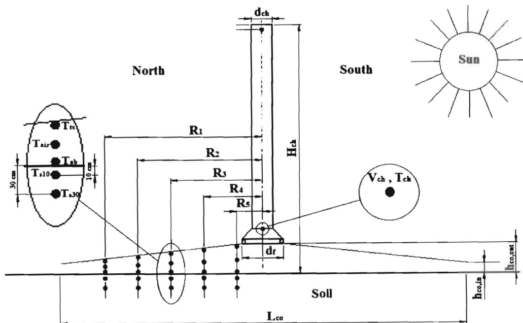
Figure 3 Schematic diagram of solar chimney with the measuring positions
