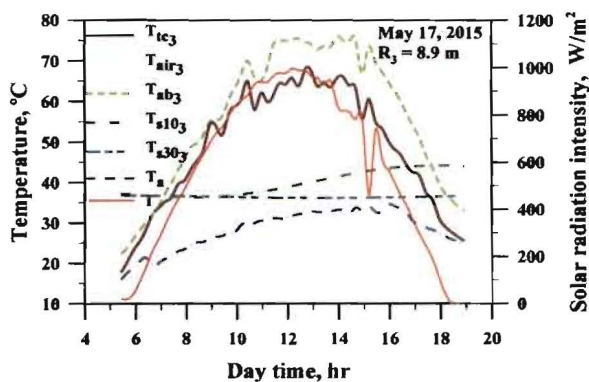
Figure 7 Temperature sensors records at R_3=8.9 m on May 17, 2015
