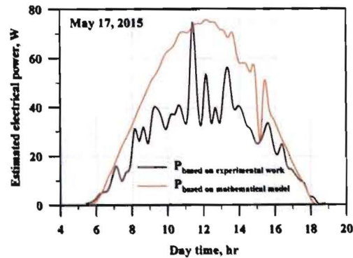
Figure 11 Predicted generated electrical power on May 17, 2015
