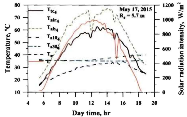
Figure 8 Temperature sensors records at R_4=5.7 m on May 17, 2015
