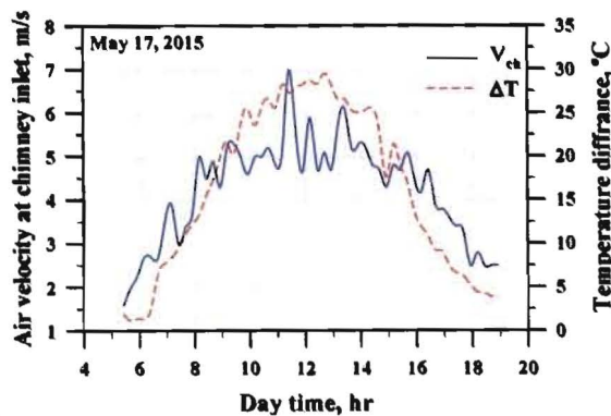
Figure 10 Air velocity at chimney inlet and temperature difference between air at chimney inlet and ambient on May 17, 2015
