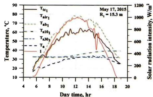
Figure 5 Temperature sensors records at R_1=15.3 m on May 17, 2015
