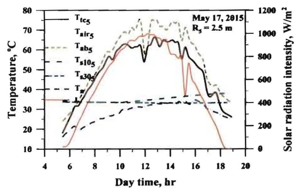
Figure 9 Temperature sensors records at R_5=2.5 m on May 17, 2015
