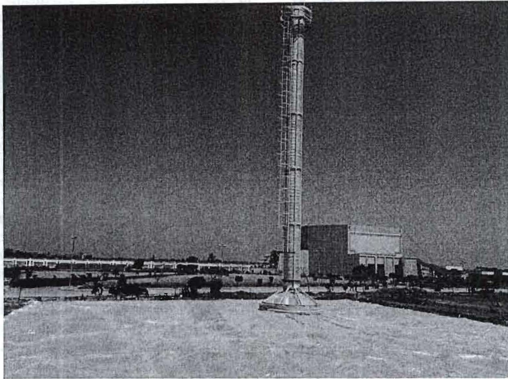
Figure 1 Photo of the experimental solar chimney pilot plant
