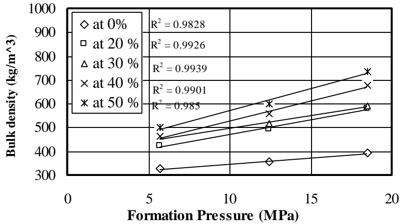
Fig. (7): Effect Of formation pressure "FP" on bulk density "Bd" (kg/m 3 ) at different binding material percentage "Bm" (%) after 7 day.
