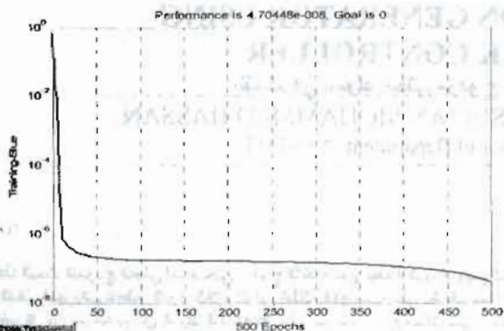
Fig 2. Training error
