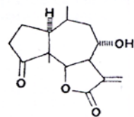
IX, Desacetylconfertiflorin
