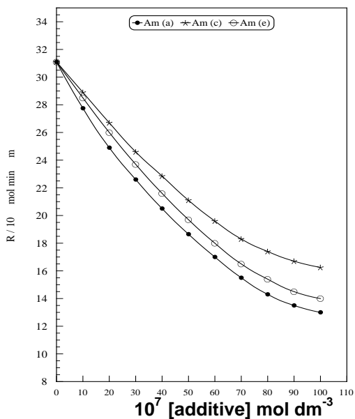
Fig.(4): Plot of rate of dissolution of COM against [additive] for different extracts of Am.
