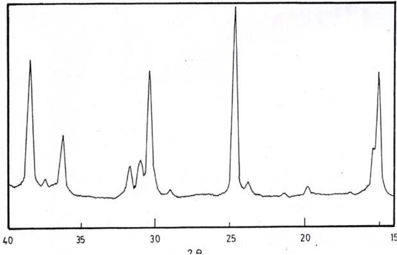
Fig. (1): X-ray powder diffraction studies for calcium oxalate crystals. IR Spectra were recorded by the IR Spectrum of Ca 2 O 4 . H 2 O fig. (2).
