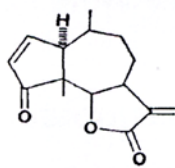
X, Ambrosin
