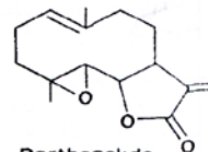
III, Parthenolide
