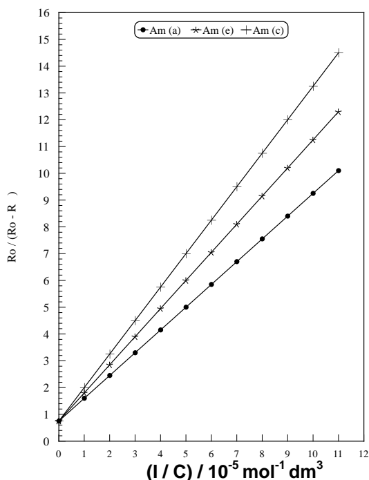
Fig.(5): Plots of R_o/R_o-R_i against (additives) of dissolution of COM in presence of Am(a),Am(e),Am(c) using emf.
