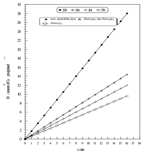
Fig. (6): Plots of amount of calcium oxalate precpitated against time in presence of some different Am extracts
