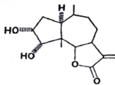
XI, Ambrosiol
