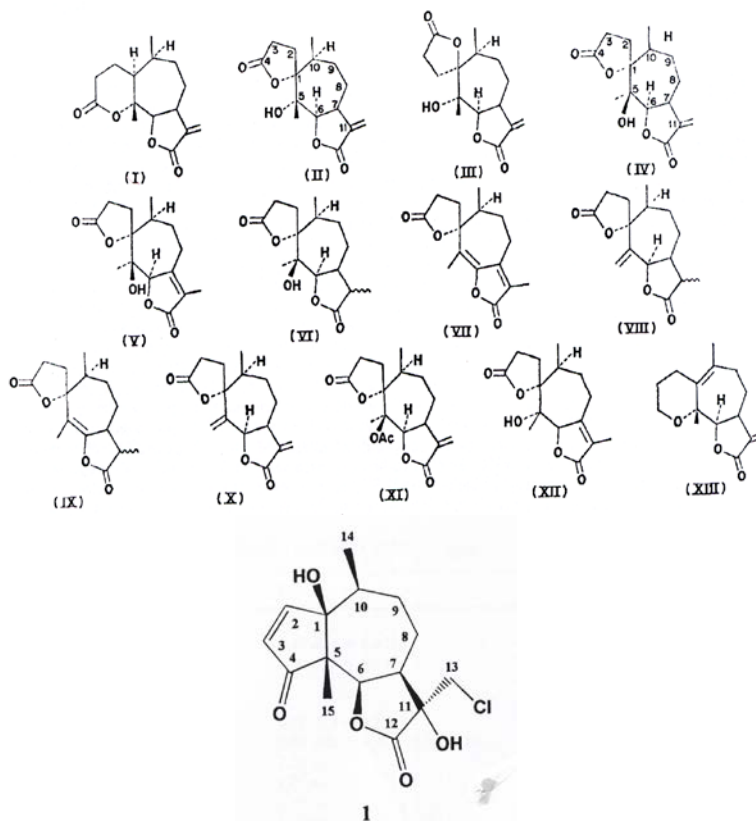
11-hydroxy-13-chloro-11,13-dihydrohymenin.
