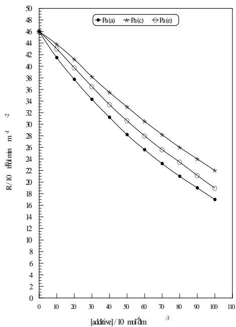
Fig. (7): Plot of rate of crystal growth of calcium oxalate against [additive] for Am(a), Am(e) and Am(c).
