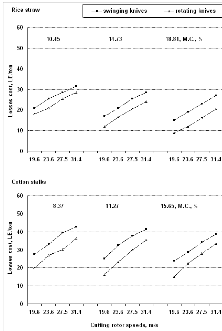
Fig. 9: Effect of cutting rotor speed and moisture on rice straw and cotton stalks losses cost under both of swinging and rotating knives.
