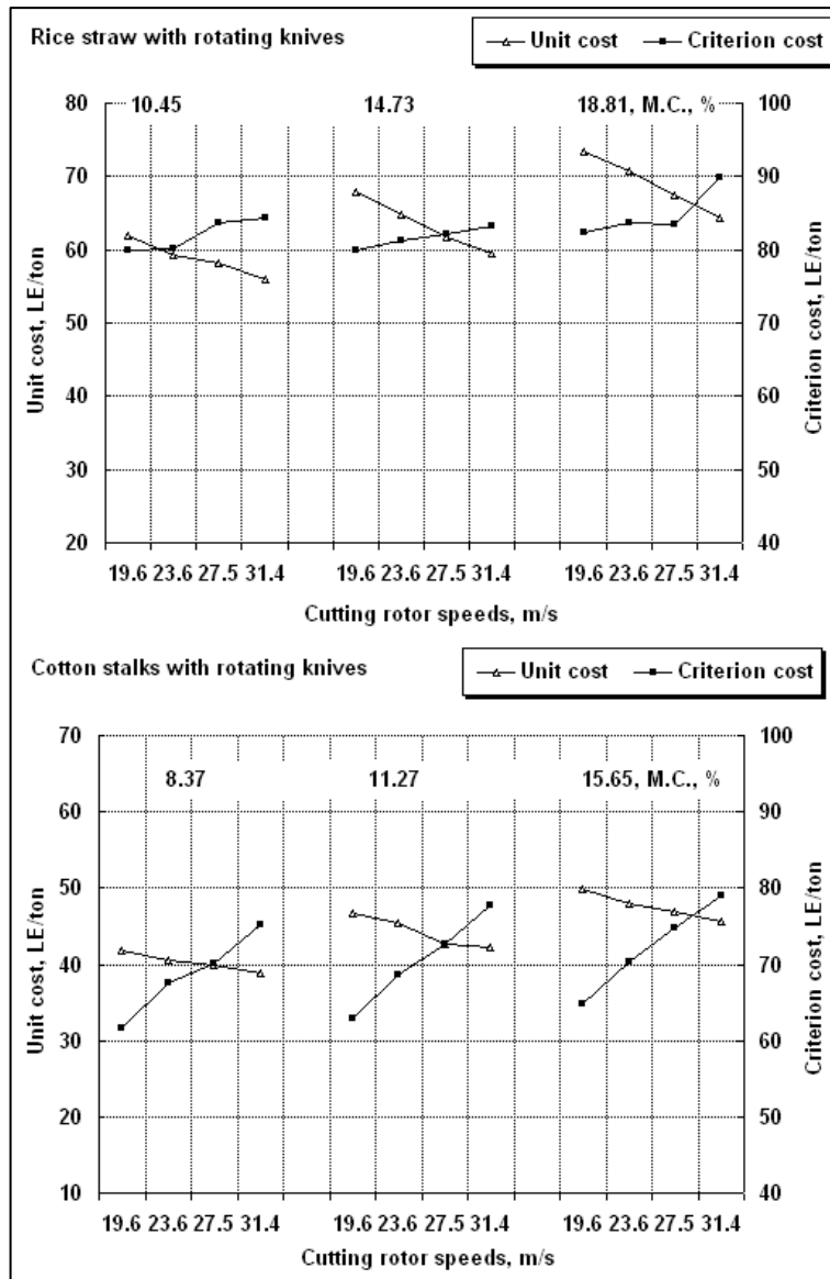
Fig. 12: Effect of cutting rotor speed and moisture content of rice straw and cotton stalks on unit and criterion function cost under rotating knives.
