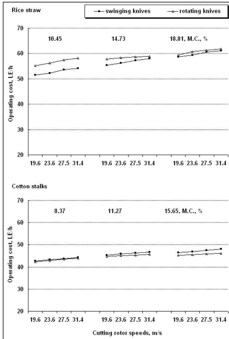
Fig. 10: Effect of cutting rotor speed and moisture on rice straw and cotton stalks operating cost under both of swinging and rotating knives.
