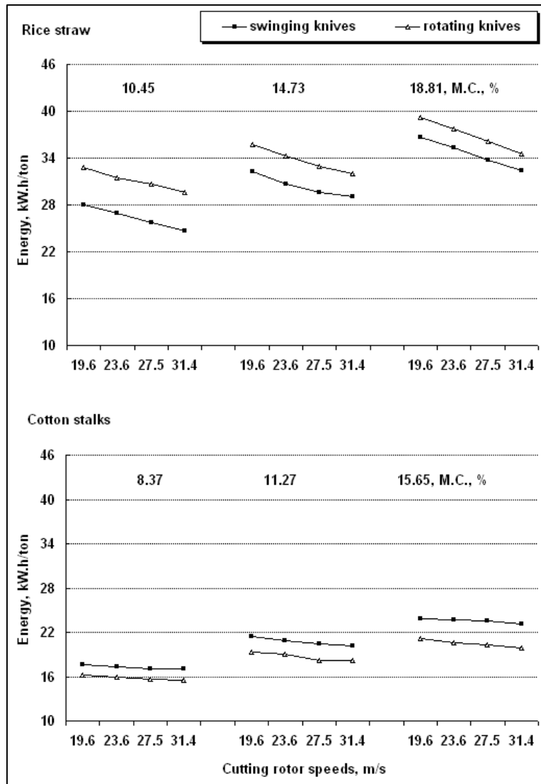
Fig. 7: Effect of cutting rotor speed and moisture on rice straw and cotton stalks energy requirements under both of swinging and rotating knives.
