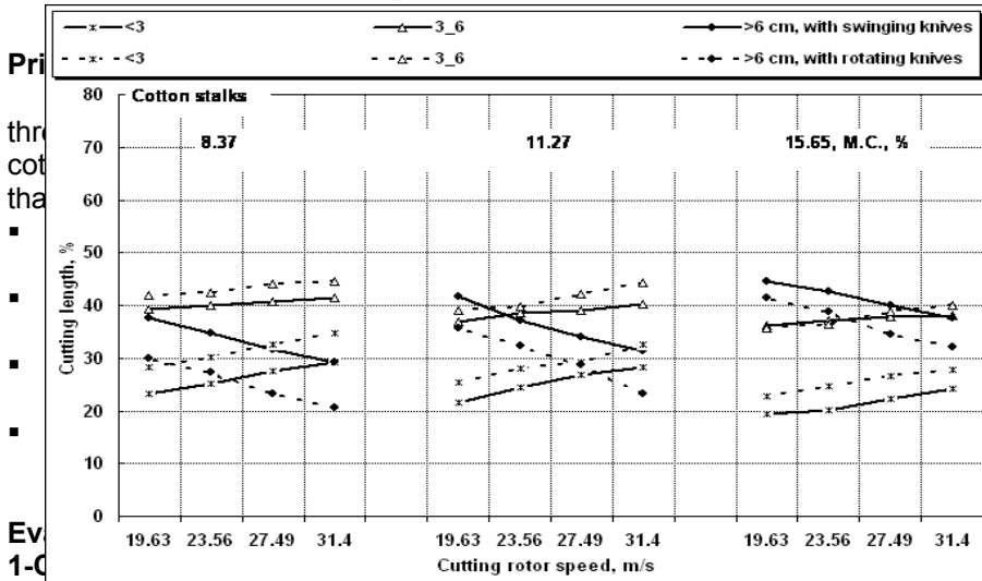
Fig. 4: Effect of cutting rotor speed and moisture content on cotton stalks cutting categories under both of swinging and rotating knives.
