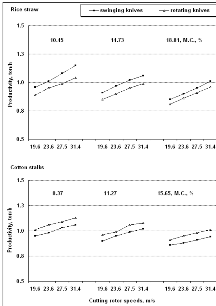
Fig. 6: Effect of cutting rotor speed and moisture content on rice straw and cotton stalks productivity under both of swinging and rotating knives.
