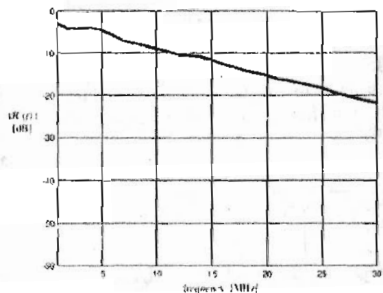
Figure 12 The frequency response of the RC1 channel
