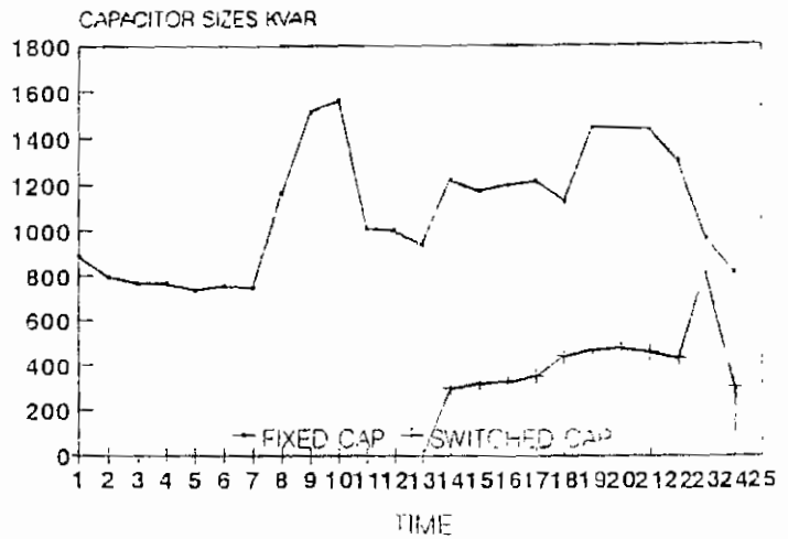
Fig.(5) Optimum size of fixed and switched capacitor banks located at sections No. 4 and 8 for switching time 11 hours.
