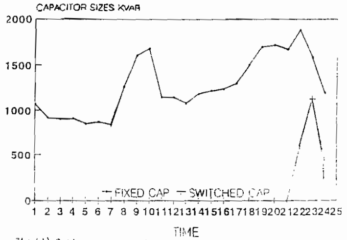
Fig.(4) Optimum size of fixed and switched capacitor banks located at sections No. 3 and 7 for switching time 3 hours.
