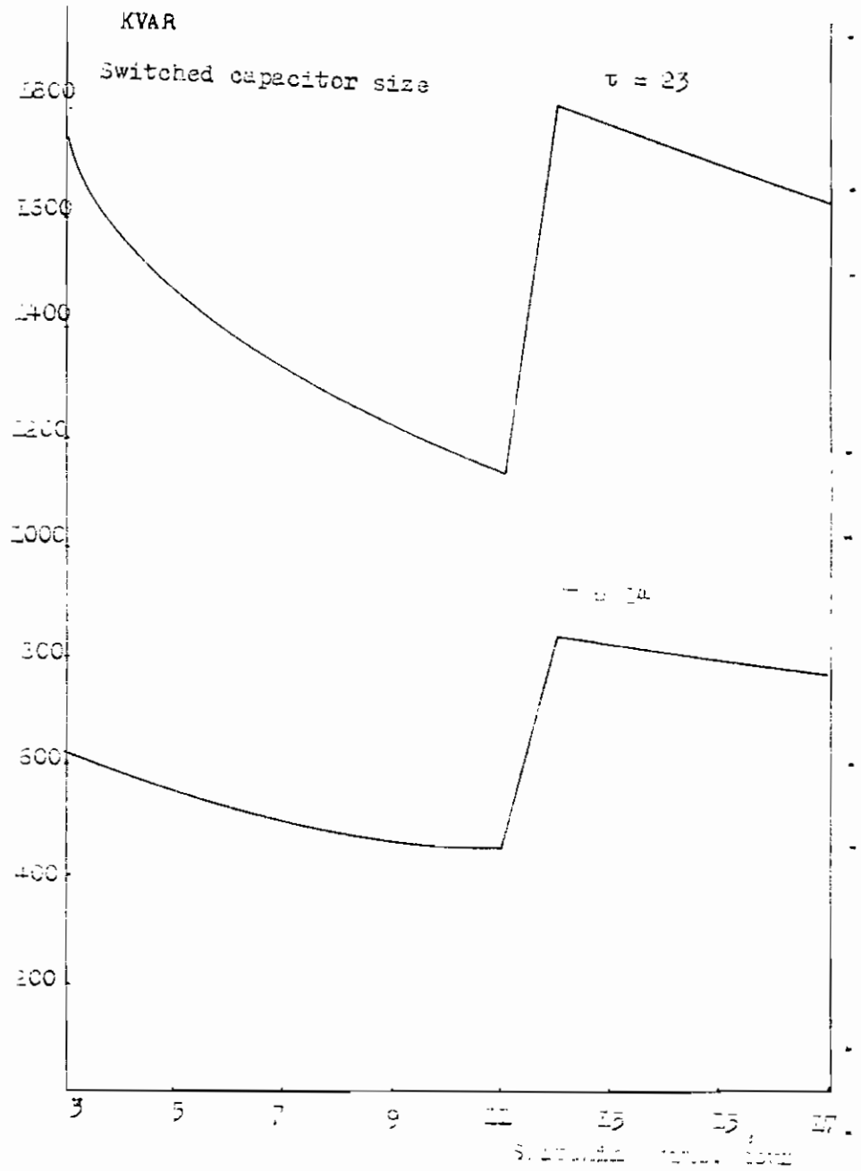
Fig. 11 Switched capacitor size against switching time, fixed capacitor locates at section 3 and switched capacitor at 4.
