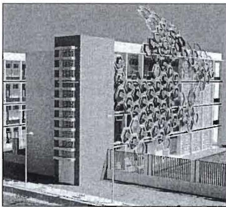
Figure 12: Visualization of the proposed BIPV system on the South facade.
