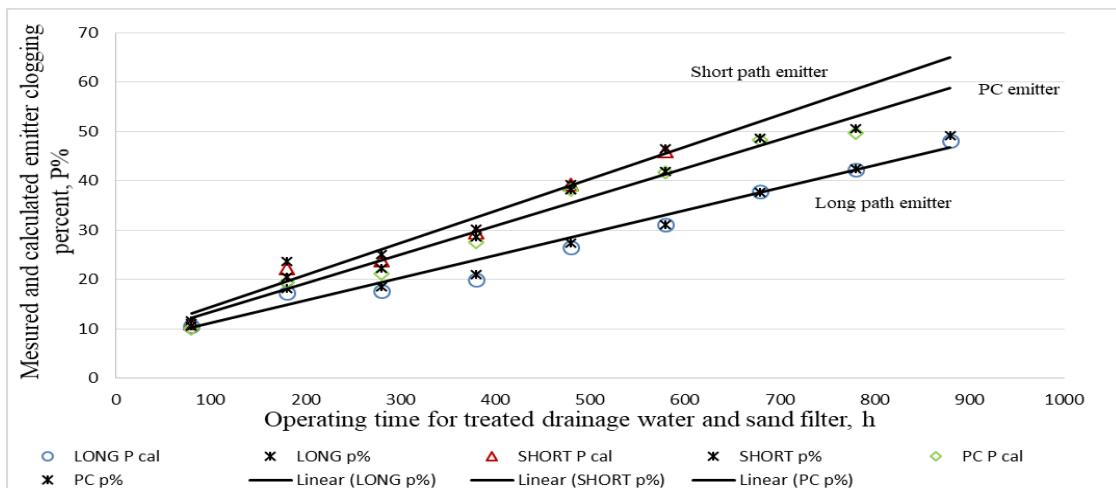
Fig (5.b): The emitter clogging percent theoretical and calculated relationship for treated drainage water and first filtration process.
